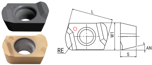
High feed insert for unfavorable conditions
